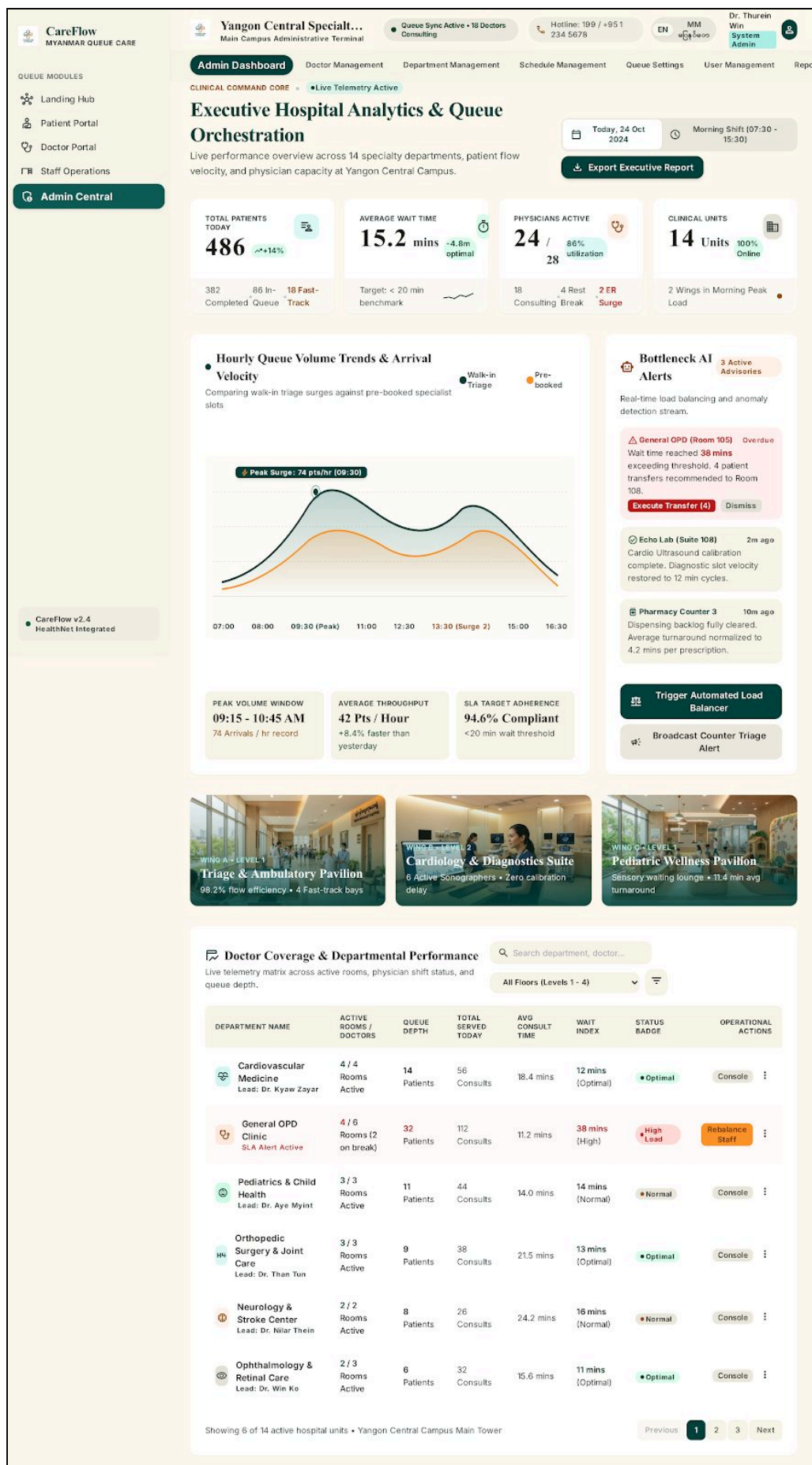
Figure 2: Administrator Dashboard
